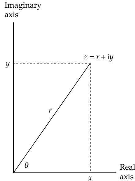
Fig. B2.6 The complex plane.
