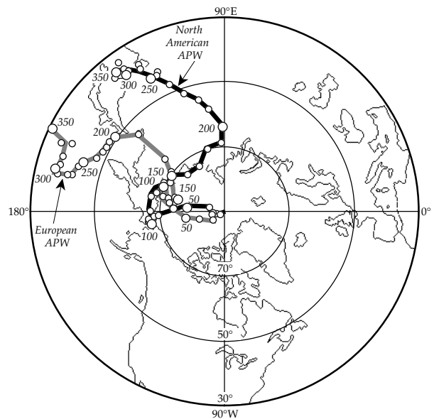
Fig. 5.66 Average apparent polar wander paths for North America and Europe in the past 350 Ma (after Irving, 1977). Numbers on paths are age in Ma.
