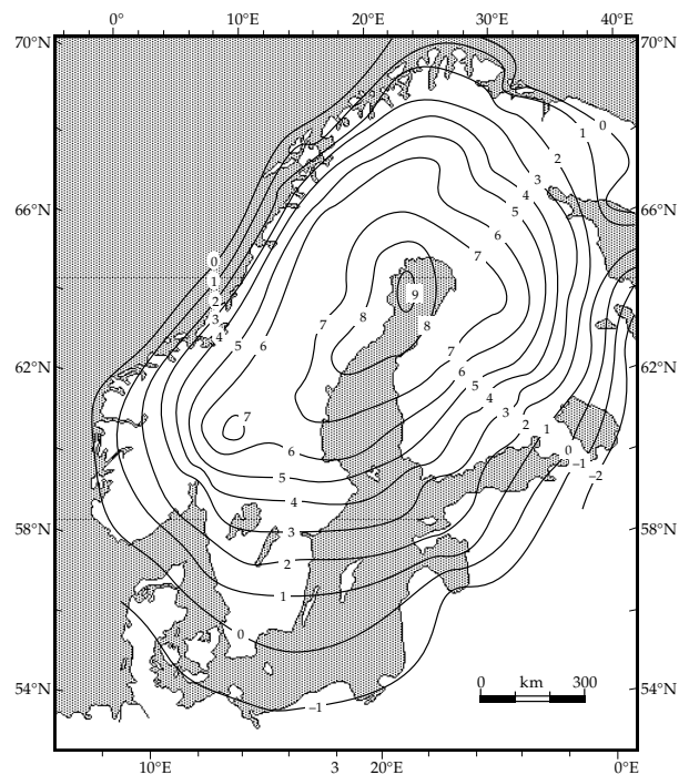
Fig. 2.66 Fennoscandian rates of vertical crustal movement (in mm yr -1 ) relative to mean sea-level. Positive rates correspond to uplift, negative rates to subsidence (after Kakkuri, 1992).
