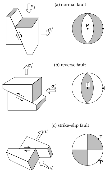
Fig. 3.37 The three main types of fault and their focal mechanisms.
