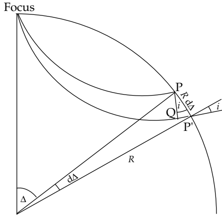
Fig. 3.80 Paths of two rays that leave an earthquake focus at infinitesimally different angles, reaching the surface at points P and P' at epicentral distances \Delta and \Delta + d\Delta , respectively.
