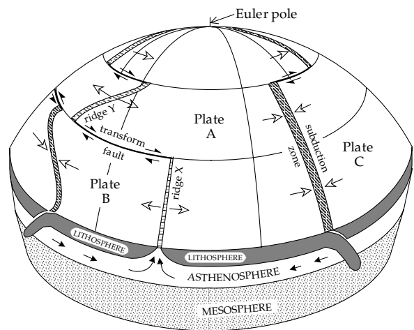
Fig. 1.12 Schematic model illustrating the three types of plate margin. Lightly hachured areas symbolize spreading ridges (constructive margins); darker shaded areas denote subduction zones (destructive margins); dark lines mark transform faults (conservative margins). The figure is drawn relative to the pole of relative motion between plates A and B. Small arrows denote relative motion on transform faults; large arrows show directions of plate motion, which can be oblique to the strike of ridge segments or subduction zones. Arrows in the asthenosphere suggest return flow from destructive to constructive margins.
